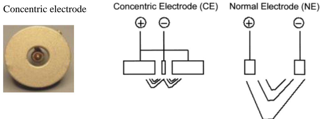
Figure 2.1: New concentric electrode (CE) and the normal electrode (NE).
